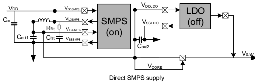
Figure 4-3. External components for SMPS step-down converter
